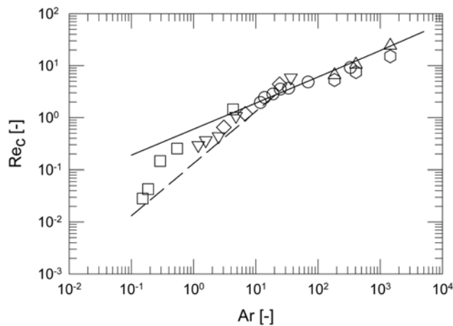
Fig. 2. Re_c versus Ar . Chehbouni et al. [5]: ( \diamond ) FCC-air, 78 \mu\text{m} , 1,450 \text{ kg/m}^3 , d_c=0.2 \text{ m} ; ( \triangle ) sand-air, 250 \mu\text{m} , 2,650 \text{ kg/m}^3 , d_c=0.2 \text{ m} ; ( \circ ) sand-air, 250 \mu\text{m} , 2,650 \text{ kg/m}^3 , d_c=0.082 \text{ m} . Peeler et al. [6]: ( \circ ) sand- \text{N}_2 , 130 \mu\text{m} , 4,400 \text{ kg/m}^3 ; ( \nabla ) alumina- \text{N}_2 , 70 \mu\text{m} , 2,800 \text{ kg/m}^3 ; ( \square ) alumina-He, 70 \mu\text{m} , 2,800 \text{ kg/m}^3 . Correlations of Choi et al. [7]: (—) Eq. (3) for Ar > 20.87 ( d_{bmax} < d_{beq} ), (---) Eq. (4) for Ar < 20.87 ( d_{bmax} > d_{beq} ).
