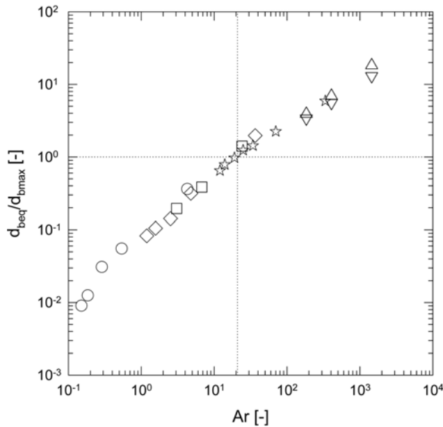
Fig. 1. d_{beq}/d_{bmax} versus Ar at u_c . Chehbouni et al. [5]: ( \square ) FCC-air, 78 \mu\text{m} , 1,450 \text{ kg/m}^3 , d_c=0.2 \text{ m} ; ( \triangle ) sand-air, 250 \mu\text{m} , 2,650 \text{ kg/m}^3 , d_c=0.2 \text{ m} ; ( \nabla ) sand-air, 250 \mu\text{m} , 2,650 \text{ kg/m}^3 , d_c=0.082 \text{ m} . Peeler et al. [6]: ( \star ) sand- \text{N}_2 , 130 \mu\text{m} , 4,400 \text{ kg/m}^3 ; ( \diamond ) alumina- \text{N}_2 , 70 \mu\text{m} , 2,800 \text{ kg/m}^3 ; ( \circ ) alumina-He, 70 \mu\text{m} , 2,800 \text{ kg/m}^3 .
